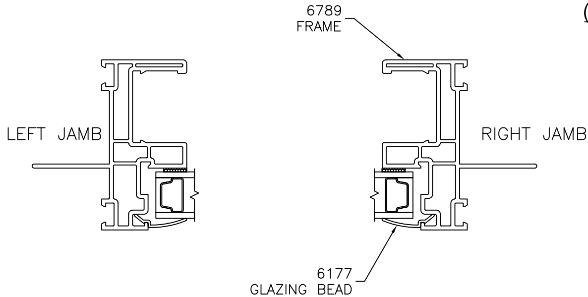
HORIZONTAL SECTION (FIXED - LITE)
