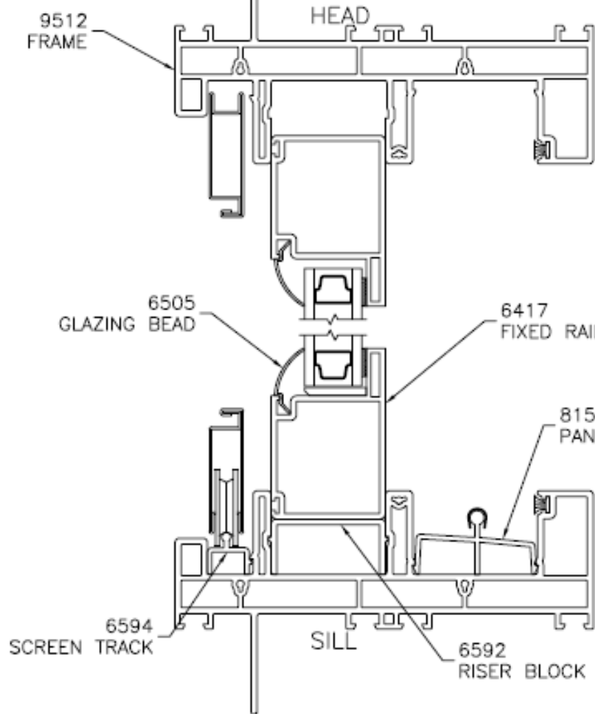
VERTICAL SECTION (FIXED PANEL)
