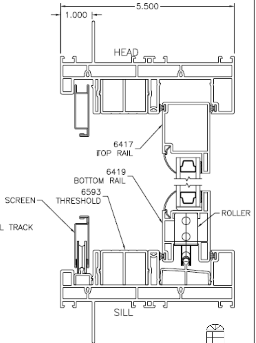
VERTICAL SECTION (OPERATING PANEL)
