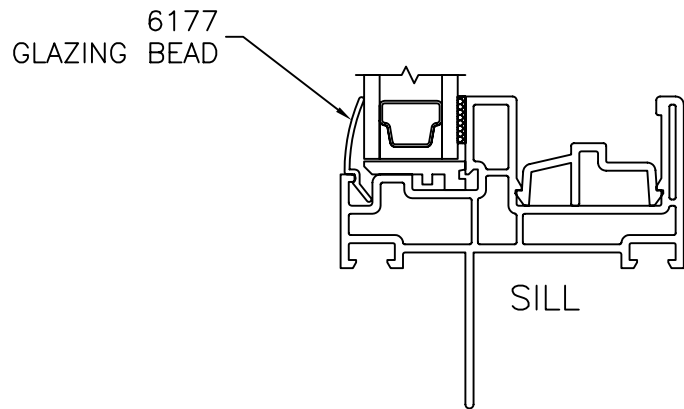
VERTICAL SECTION (FIXED - LITE)
