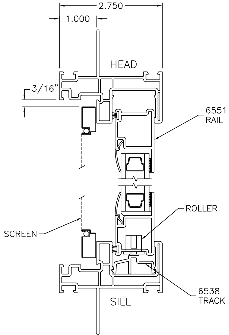
VERTICAL SECTION (VENT - LITE)
