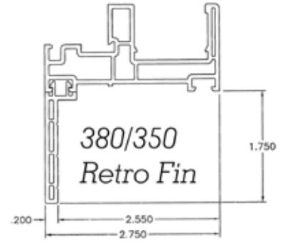
CASEMENT WINDOWS
