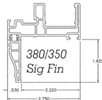
CASEMENT WINDOWS
